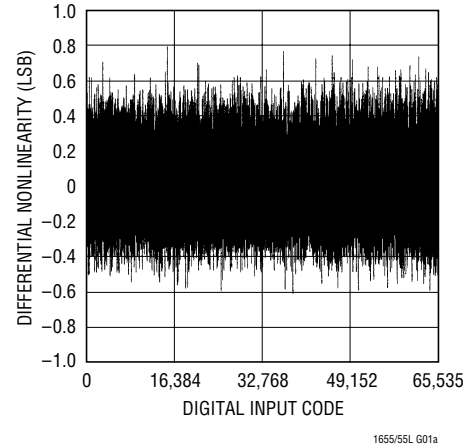
LTC1655L Differential Nonlinearity
